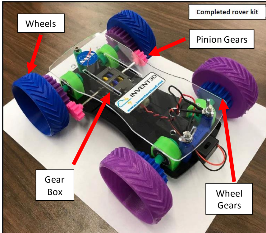
Figure 1: Diagram of Rover Components (credits to INVENTORcloud for ROVER KIT)
